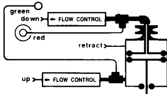
CYLINDER WITH RETRACT
