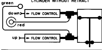
CYLINDER WITHOUT RETRACT
